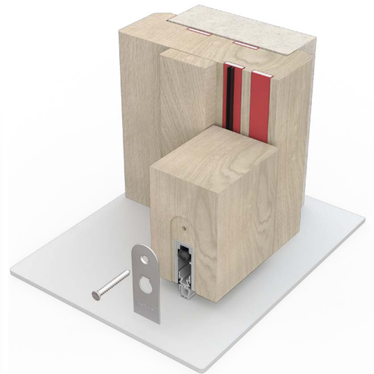
FD60 example: TS seal (Shown with with LP1504 fire seal & LAS8001 si + cladding kit)
