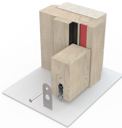
▲ FD30 example: AS seal with Batwing® to comply with BS 9999 (Shown with LAS8001 si)
